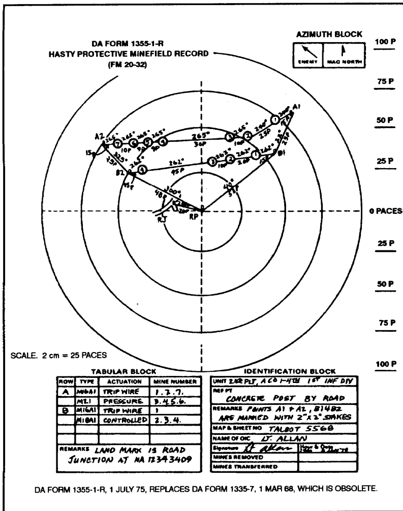
Figure 109. Marking and recording minefield (continued).
